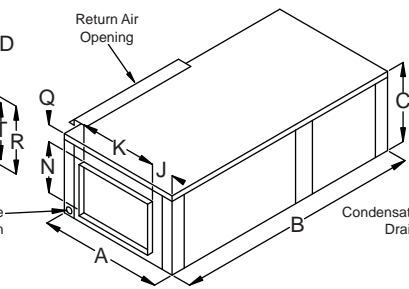
Right Hand Return End Blow (FRE)
