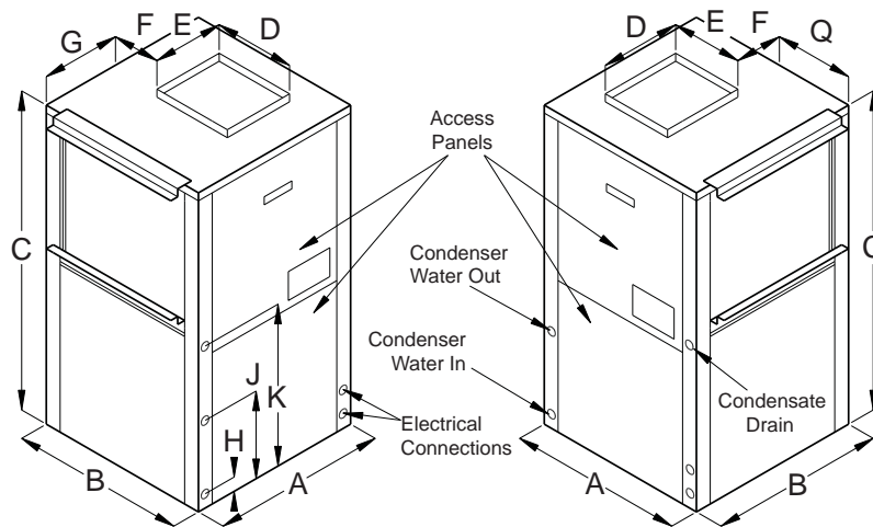
Left Hand Return (FLT)
