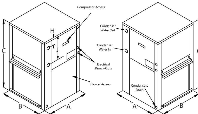
Left Hand Return (FLB)
