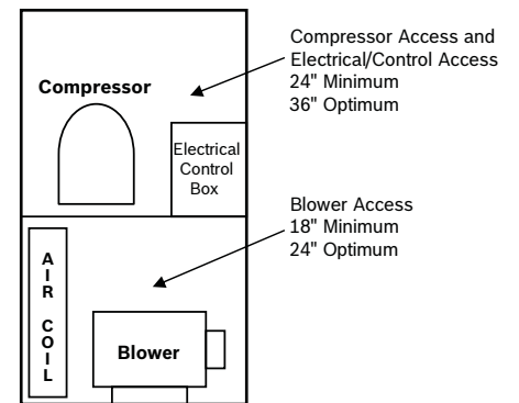
Front of Unit Service Clearances
