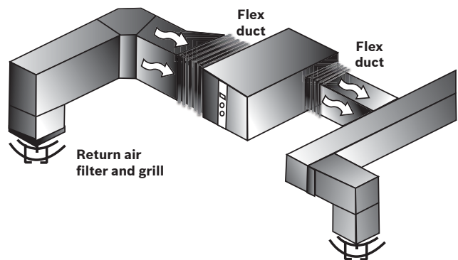
Figure 11: Return Air Ducting
