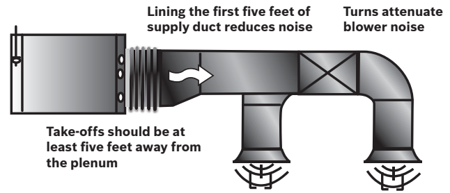
Figure 10: Supply Air Ducting
