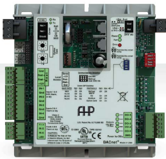
DDC Control Board
