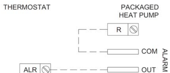
Fig. 44 Alarm Support for 24VAC Thermostats
