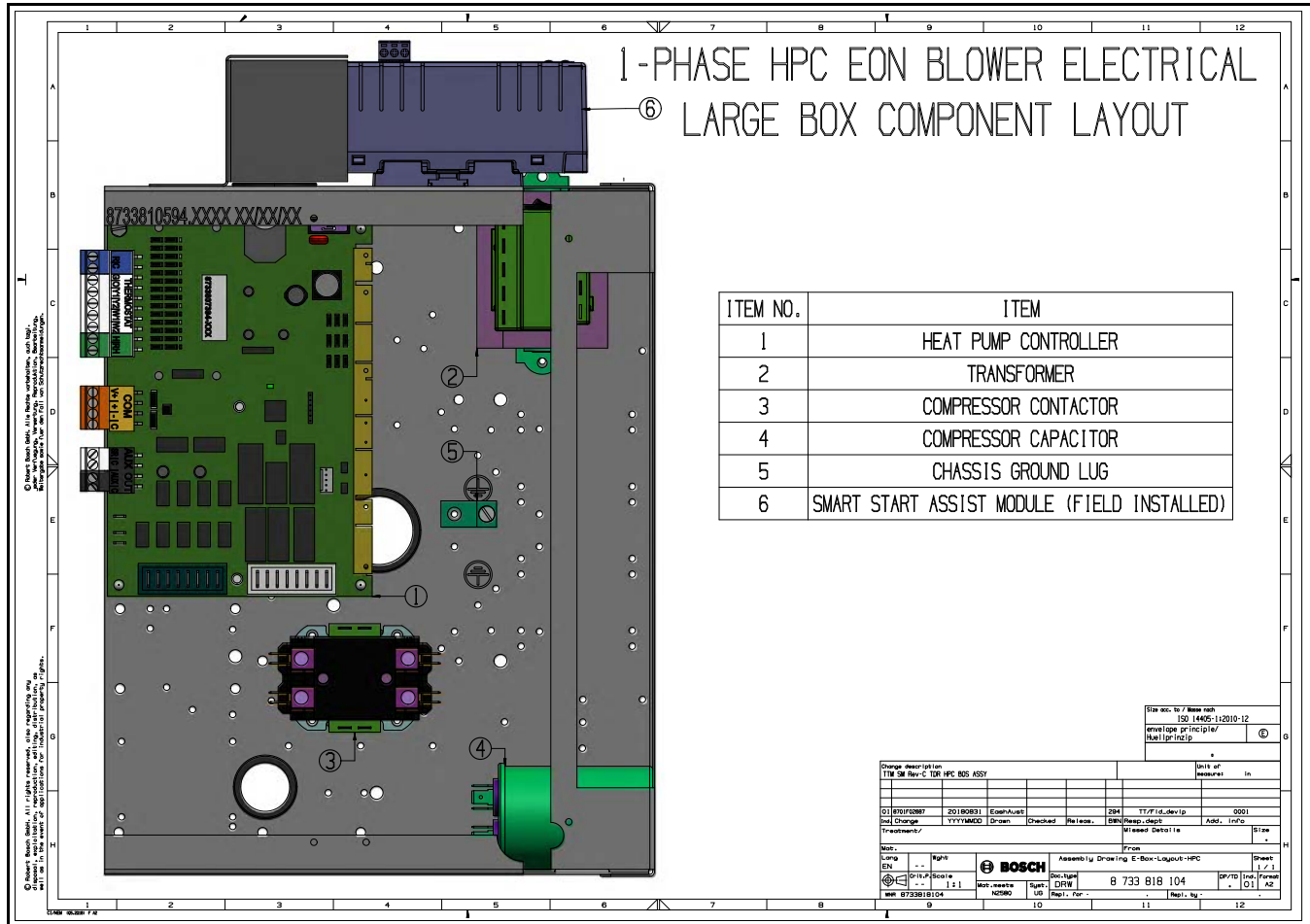
Fig. 38 Typical Electrical Box Layout
