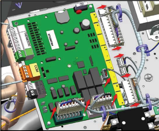
Fig. 16 HPC Wiring Disconnected
