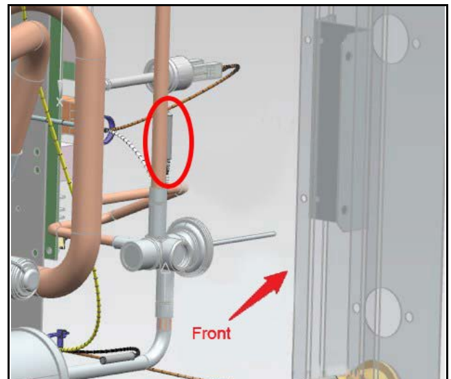
Fig. 9 FZE Sensor Locations
