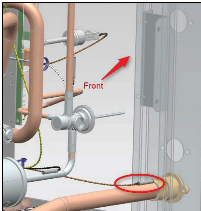
Fig. 7 EWT Sensor Location
