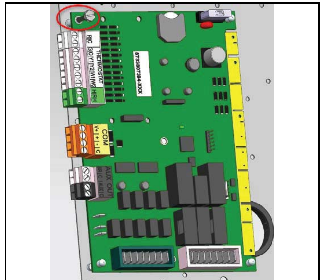
Fig. 19 Ground Screw Circled
