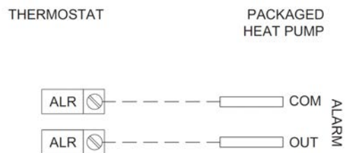
Fig. 43 Alarm Support for Dry Contact Thermostats
