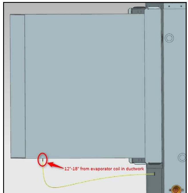
Fig. 5 RAT Sensor Field Location
