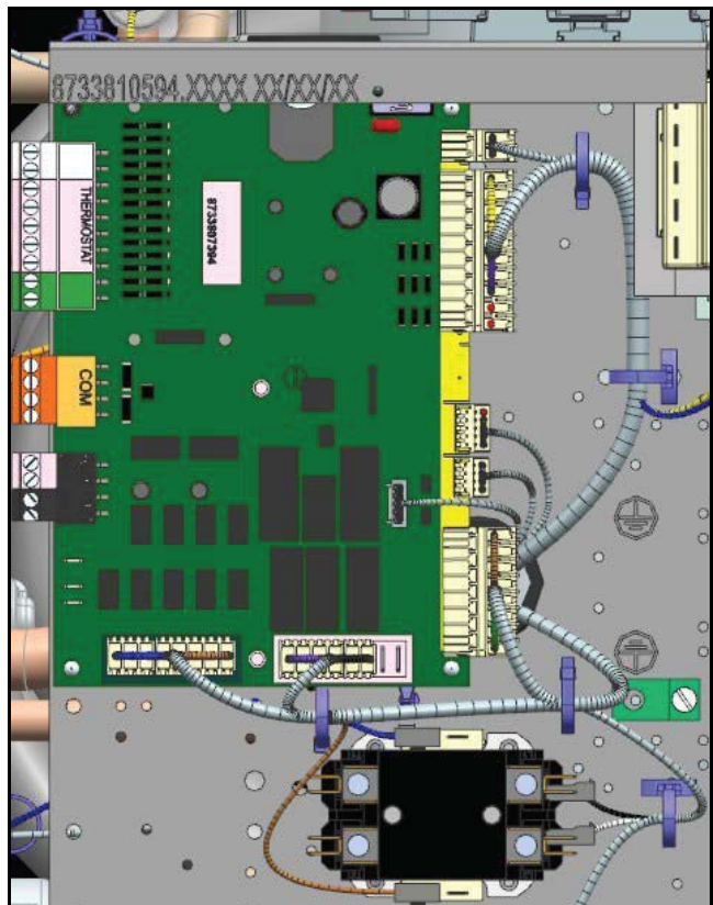
Fig. 15 HPC Harness Connections
