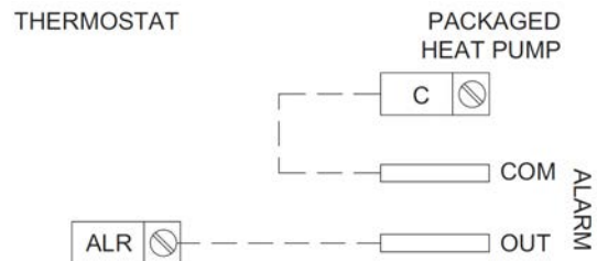
Fig. 42 Generic Thermostat Connections
