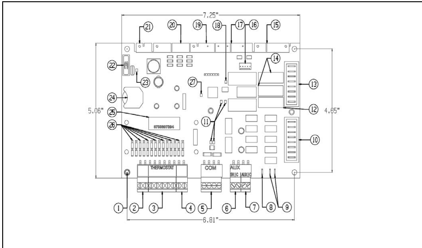
Fig. 1 Heat Pump Controller
