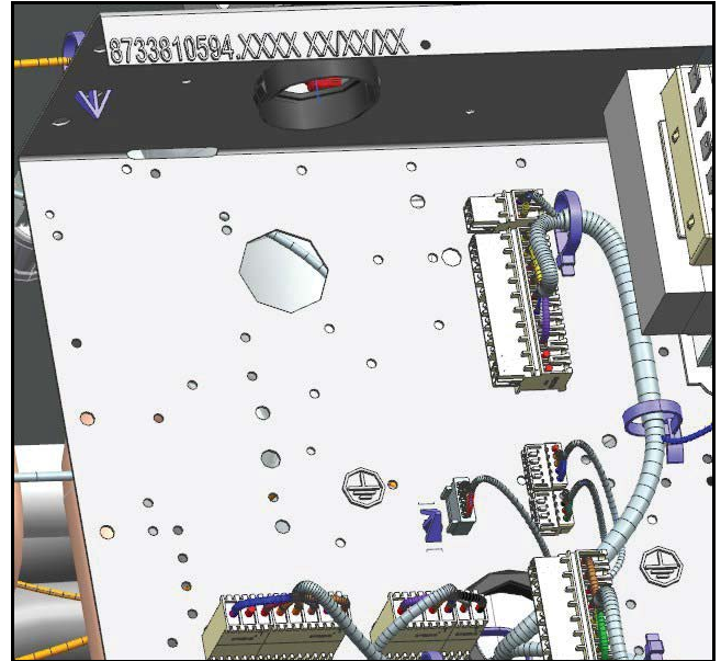
Fig. 18 HPC Board Removed
