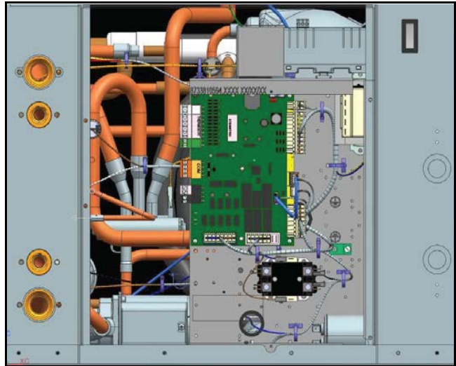
Fig. 14 Electrical Access Panel Removed
