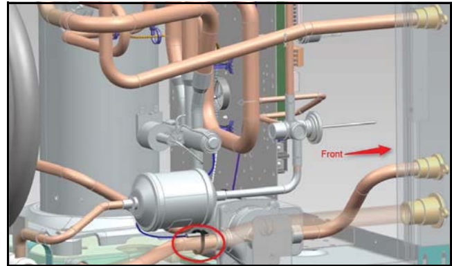
Fig. 11 DWT Sensor Location
