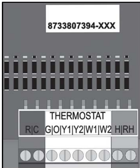
Fig. 39 HPC Thermostat Connectors
