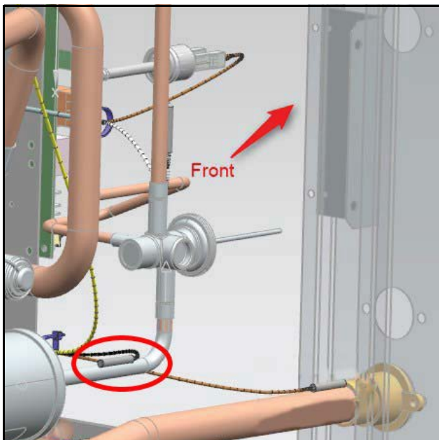
Fig. 8 FZC Location
