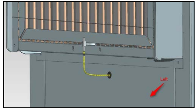
Fig. 4 RAT Sensor Factory Location
