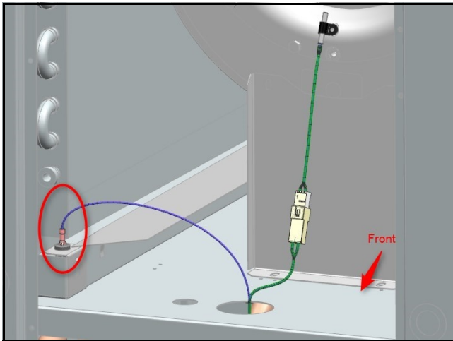
Fig. 2 Condensate Overflow Sensor Location
