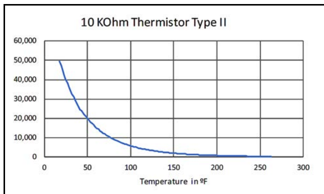
Fig. 12 Type II Thermistor Temperature Curve
