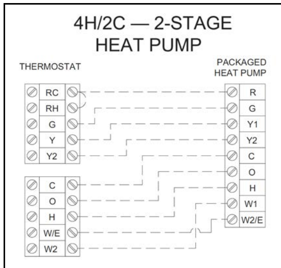
Fig. 40 Generic Thermostat Connections
