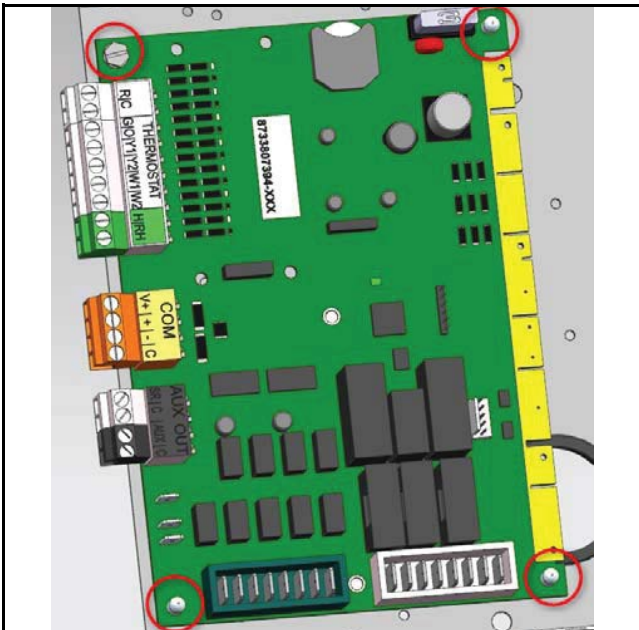
Fig. 17 Standoffs and Ground Screw
