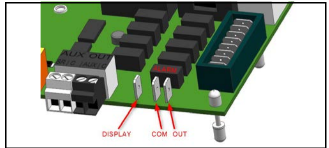
Fig. 41 Alarm Terminal Connectors on the HPC Board
