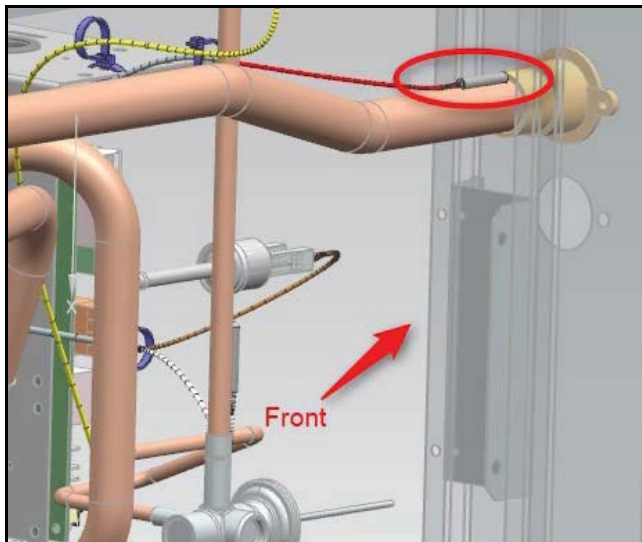
Fig. 6 LWT Sensor Location
