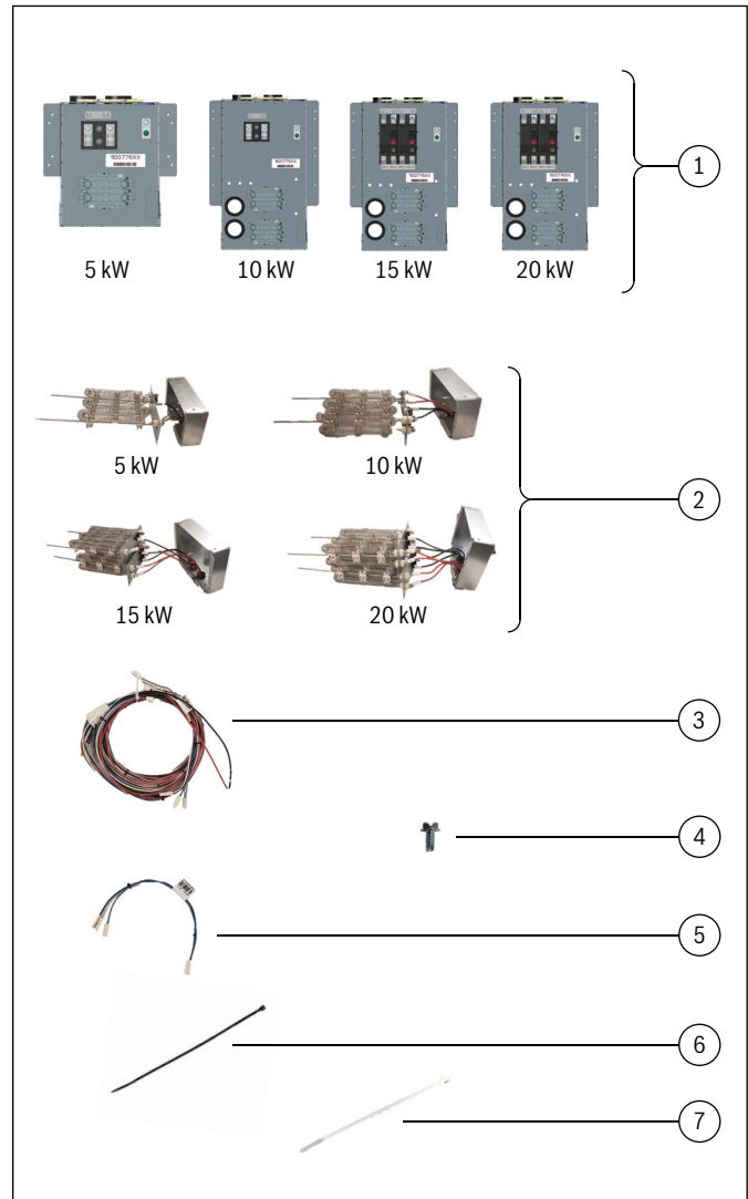
Figure 1 Kit Components
