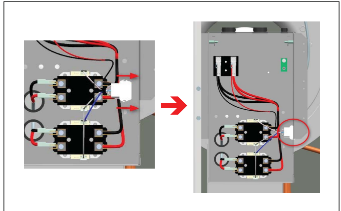
Figure 32 J39 Connector Right Hand Configuration
