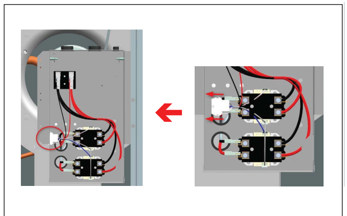
Figure 33 J39 Connector Left Hand Configuration
