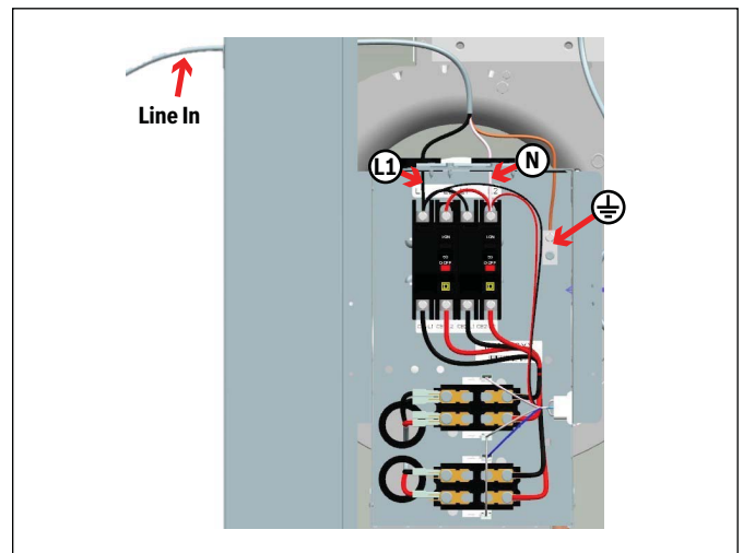
Figure 43 15kW Field Wiring - Top View
