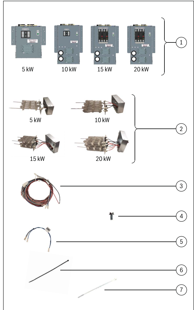
Figure 1 Kit Components
