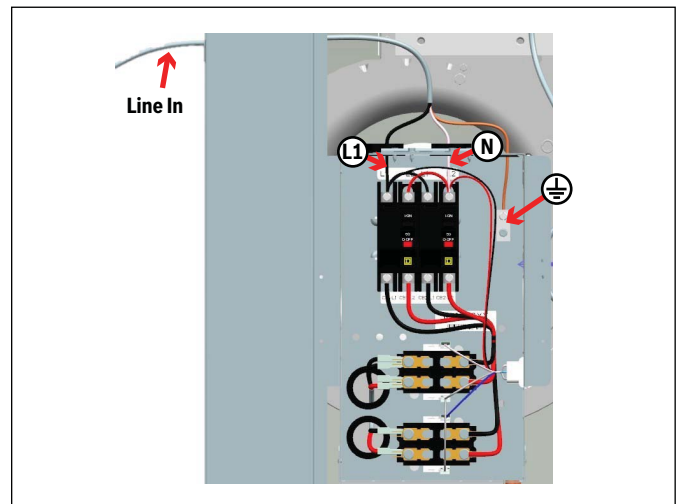
Figure 44 20kW Field Wiring - Top View
