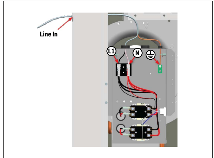
Figure 42 10kW Field Wiring - Top View
